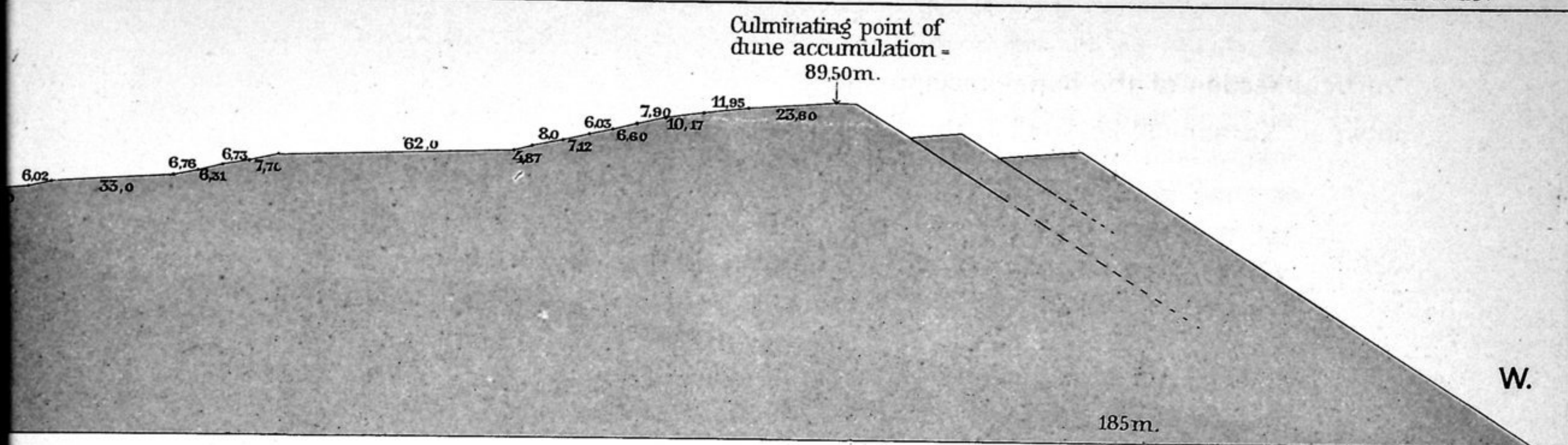
Vertical section of the southern basin of Karaunelik-köl and its dune-accumulations
