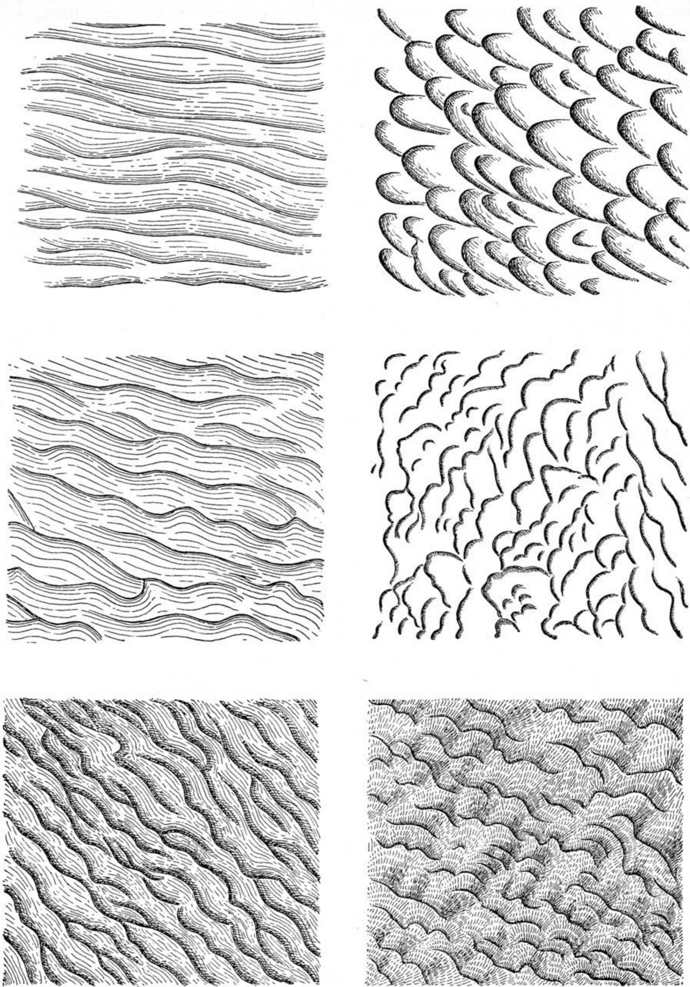
Fig. 188. DIFFERENT PATTERNS OF RIPPLE-MARKS. DESERT OF LOP.
