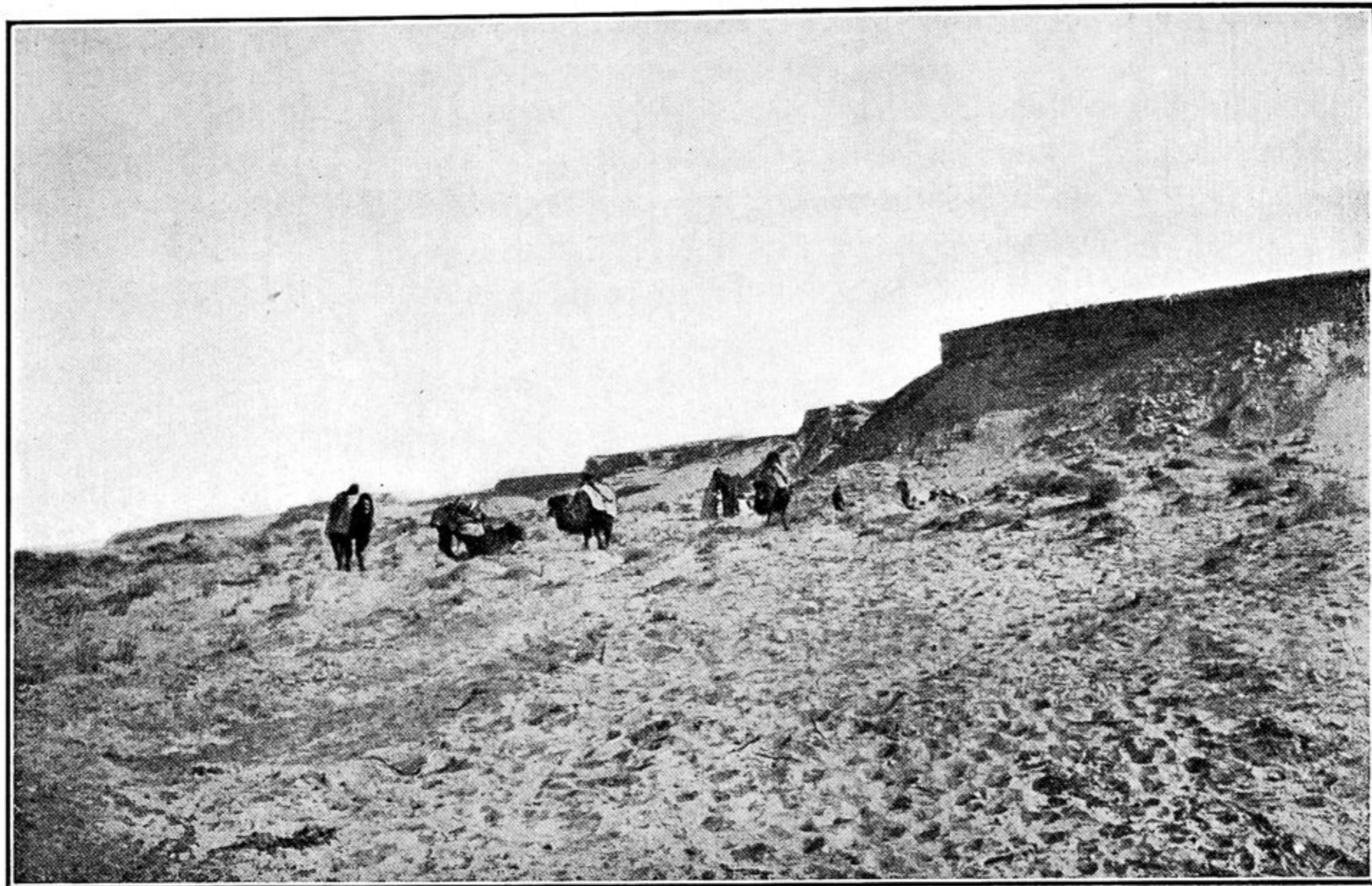
Fig. 230. ANOTHER VIEW OF THE CLAY TERRACE.
