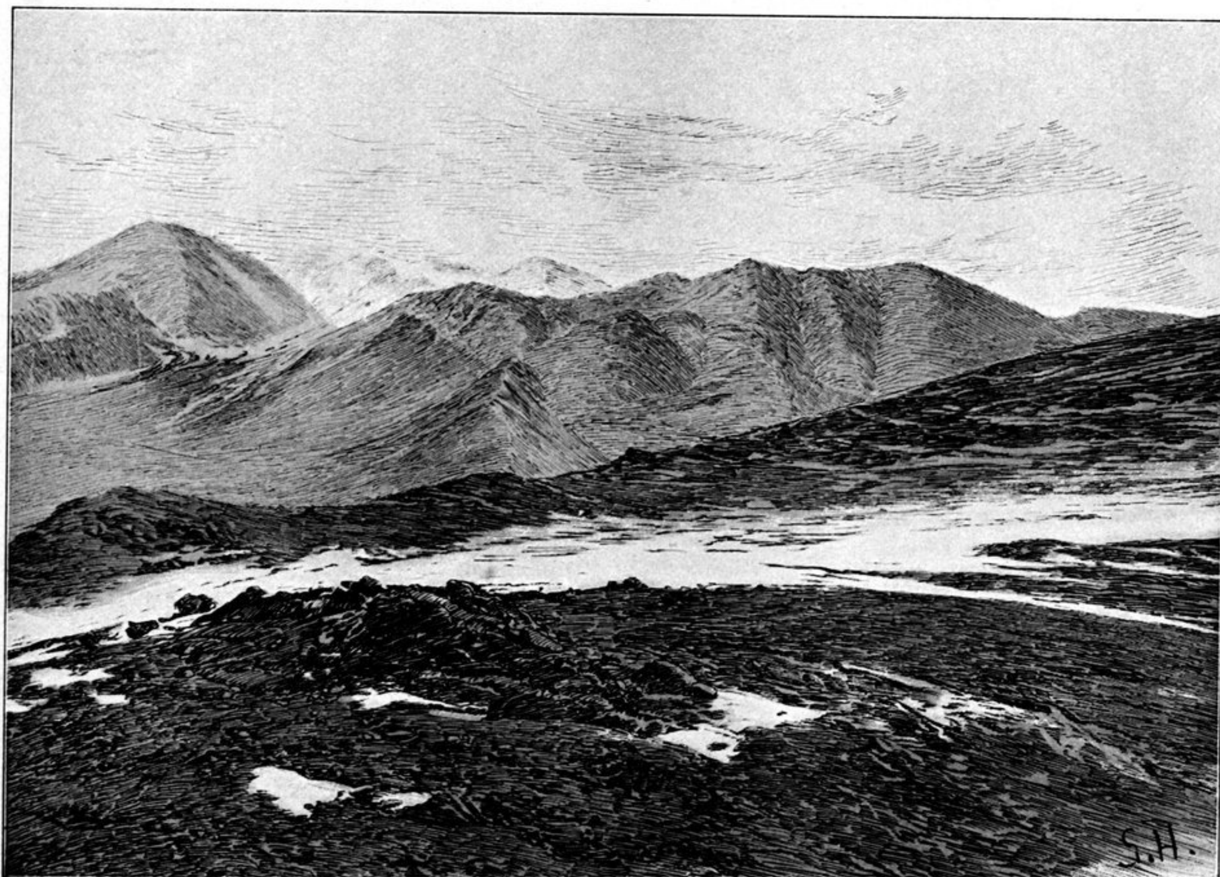
LOOKING S 66° E FROM THE LAST PANGGONG-TSO PASS.
