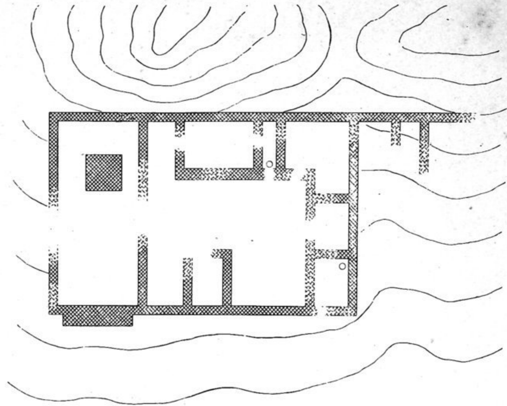
SKETCH PLAN OF SHRINE BELOW YUTÖGH
