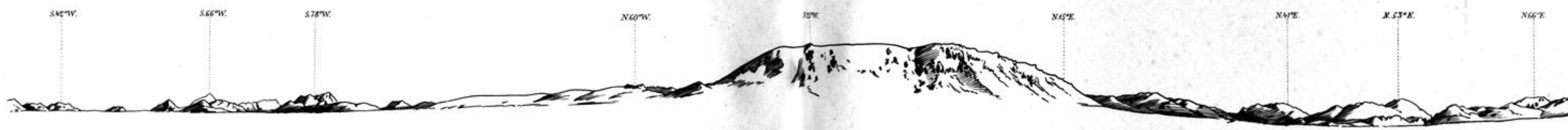
397 A. FROM CAMP 308, JAN. 19, 1908 (PL. 16)
