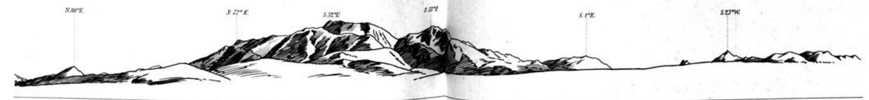
397 B. FROM CAMP 308, JAN. 19, 1908 (PL. 16)
