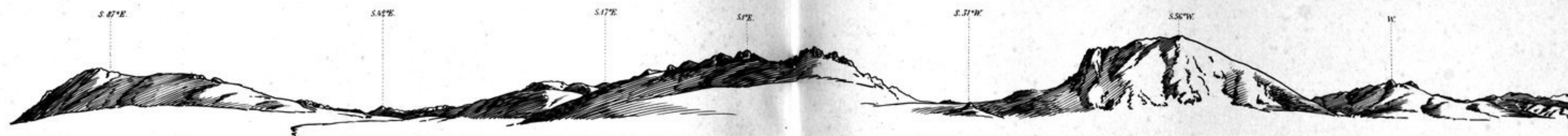
395 A. FROM CAMP 305, JAN. 15, 1908 (PL. 16)
