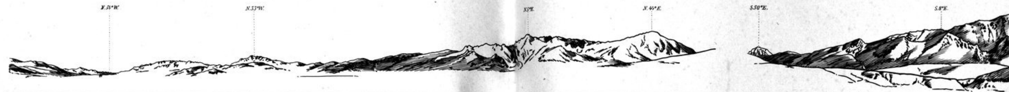
395 B. FROM CAMP 305, JAN. 15, 1908 (PL. 16)
