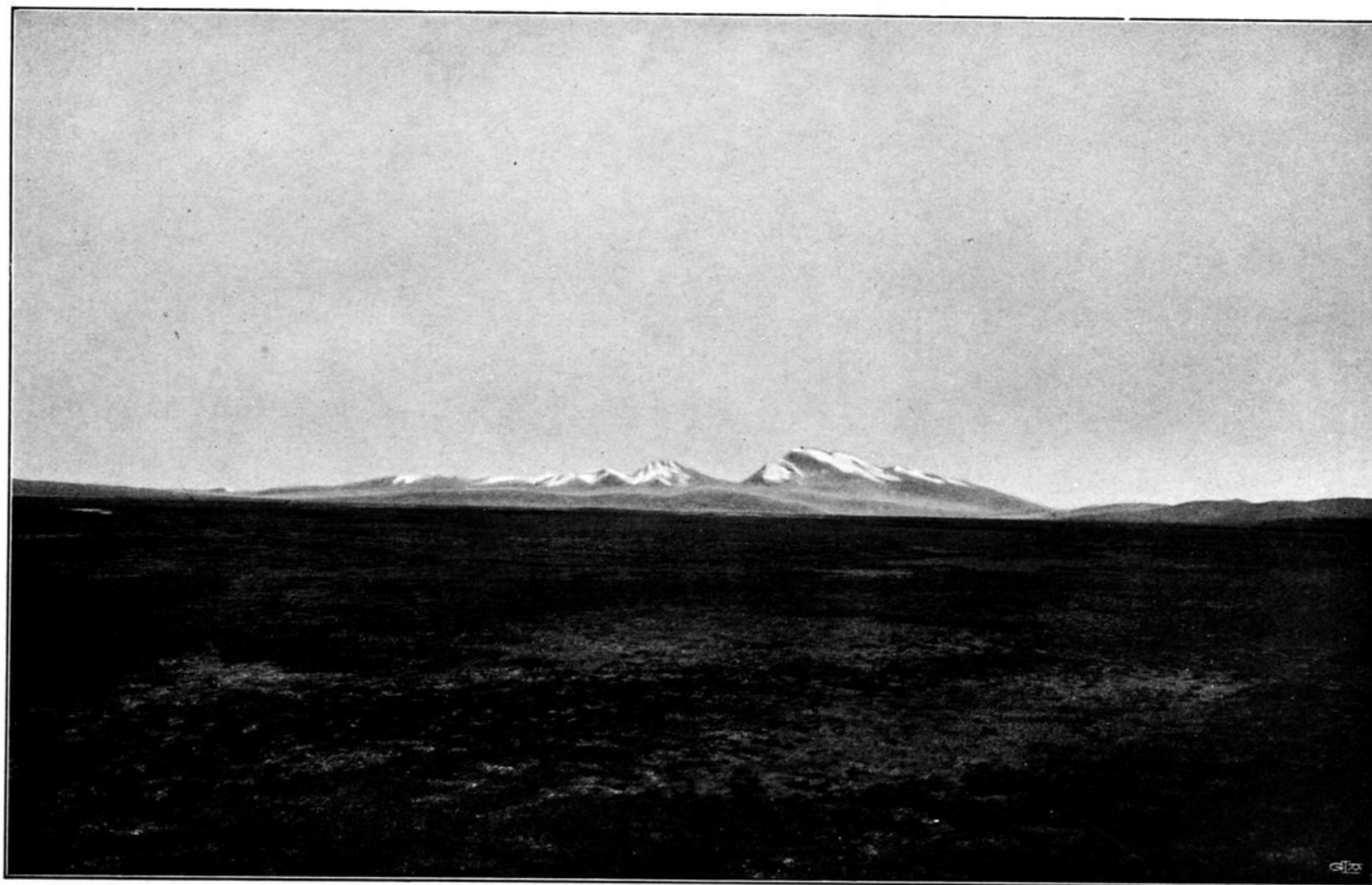
THE GURLA-MANDATA (MAMO-NANI) FROM KHALEB. HEIGHT 25355 FEET OR 7730 M (BURRARD).
