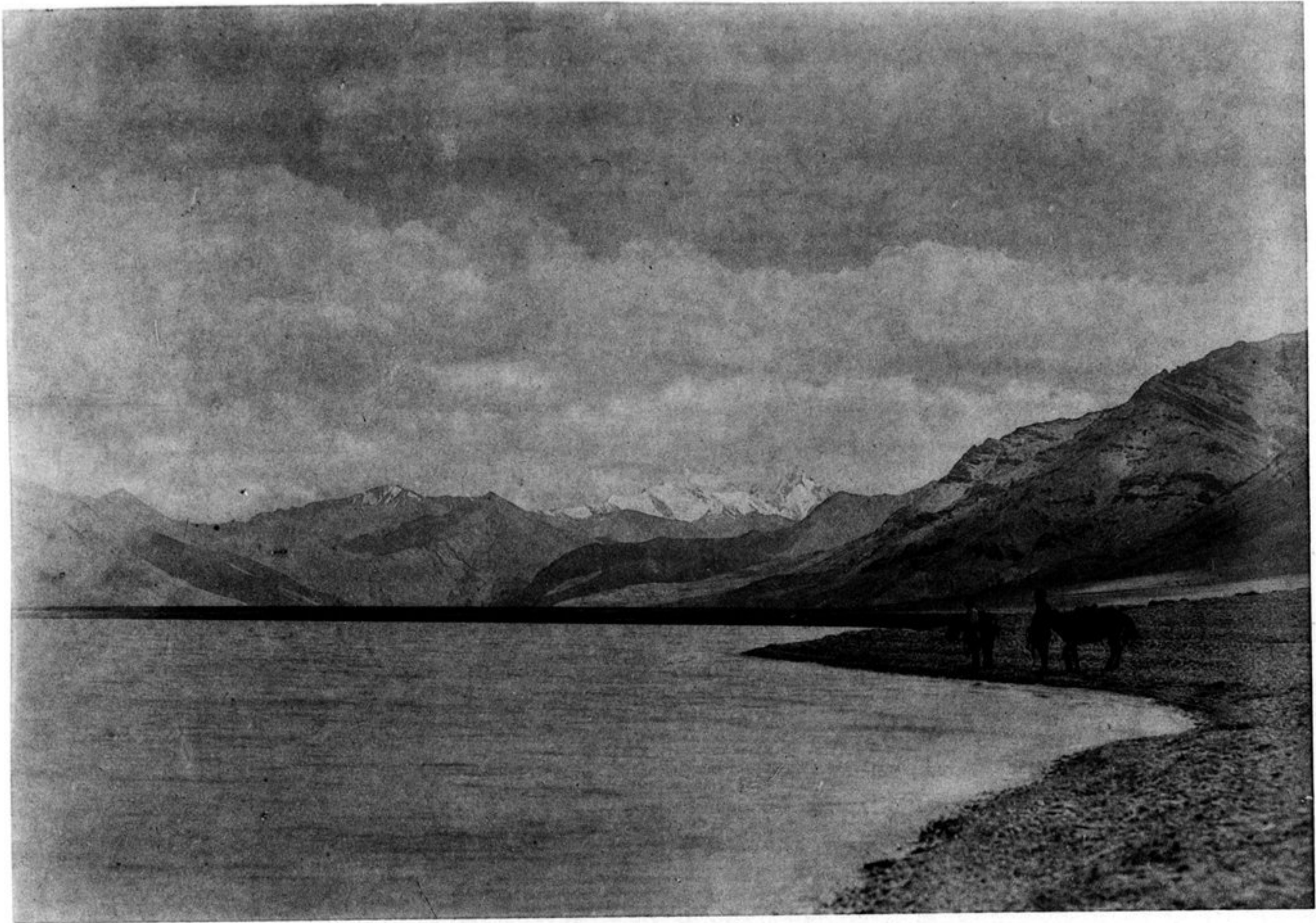
a. Lake Thsomo Riri from the north.
