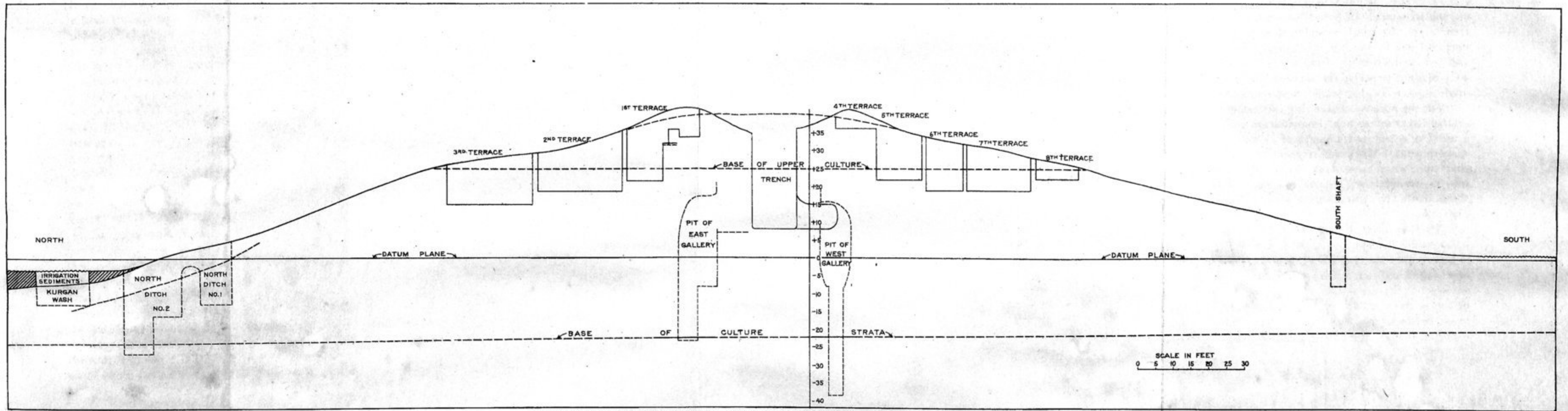
NORTH-SOUTH SECTION NORTH KURGAN, ANAU, TRANS-CASPIA. APRIL 9TH 1904. R. W. PUMPELLY.
