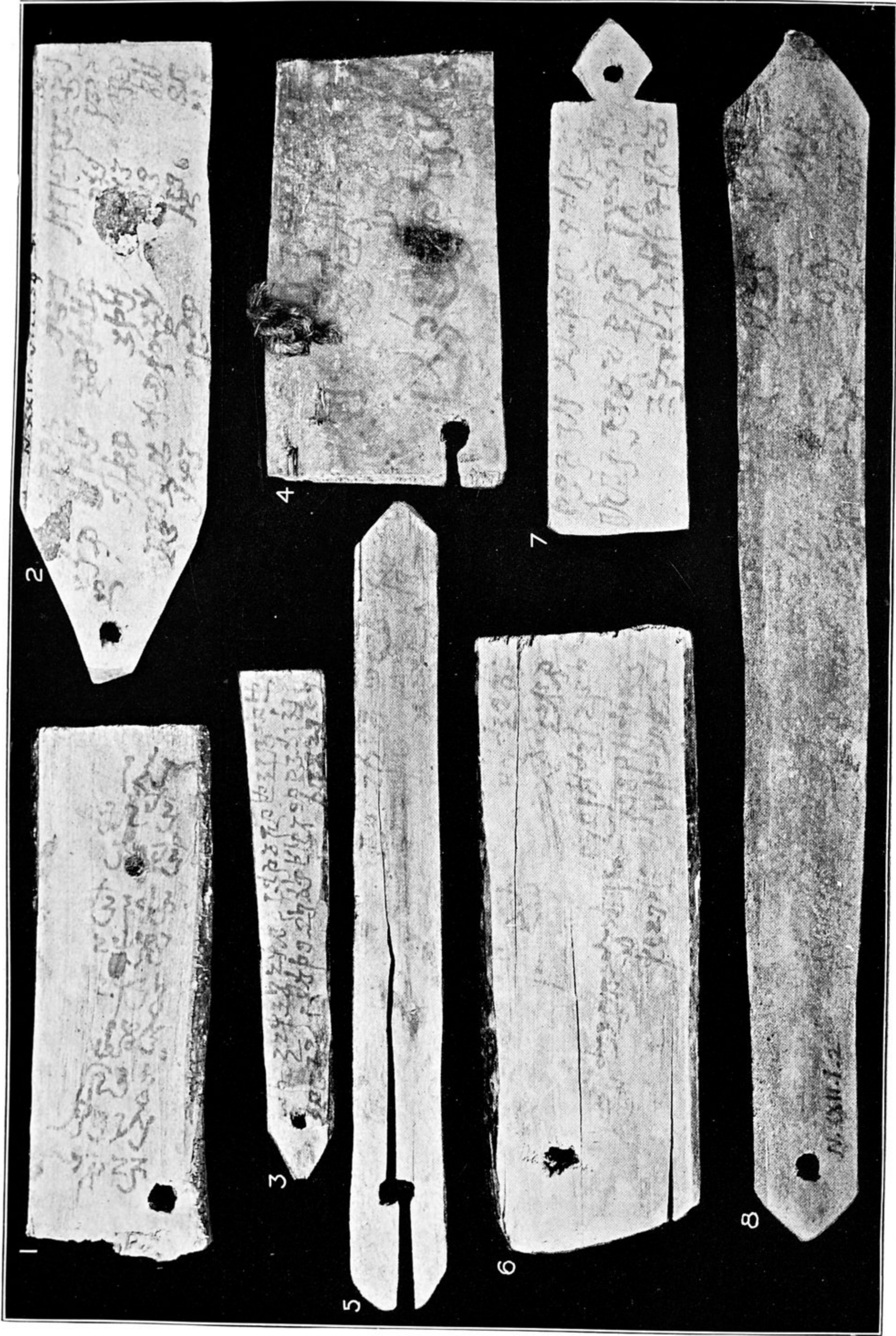
97. KHAROSHTHI RECORDS ON OBLONG AND LABEL-SHAPED WOODEN TABLETS FOUND AT NIYA SITE. Scale, one-half.
